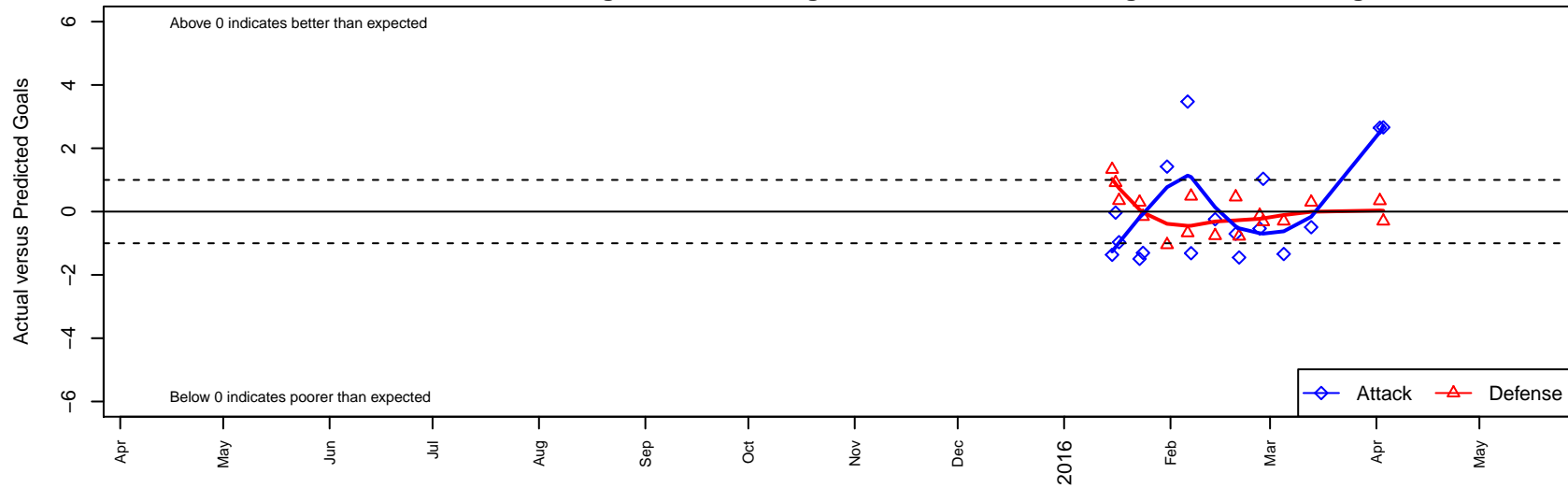
Portland Thorns Academy G99 Dots are actual minus expected GF (blue circles) and GA (red triangles). Blue line is smoothed change in attack strength. Red is smoothed change in defense strength.
